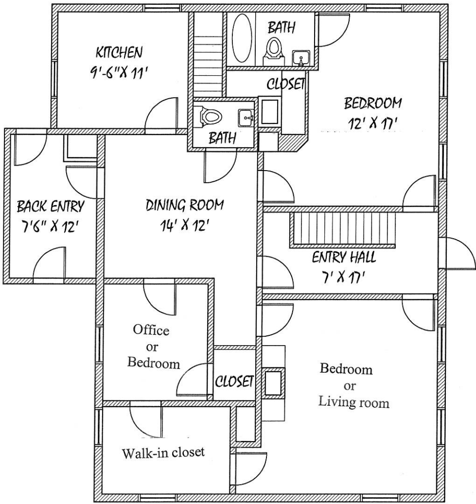
2 bedroom, 1st floor apartment in the William Gyles House Scaled drawing 1/8" = 1'0"
